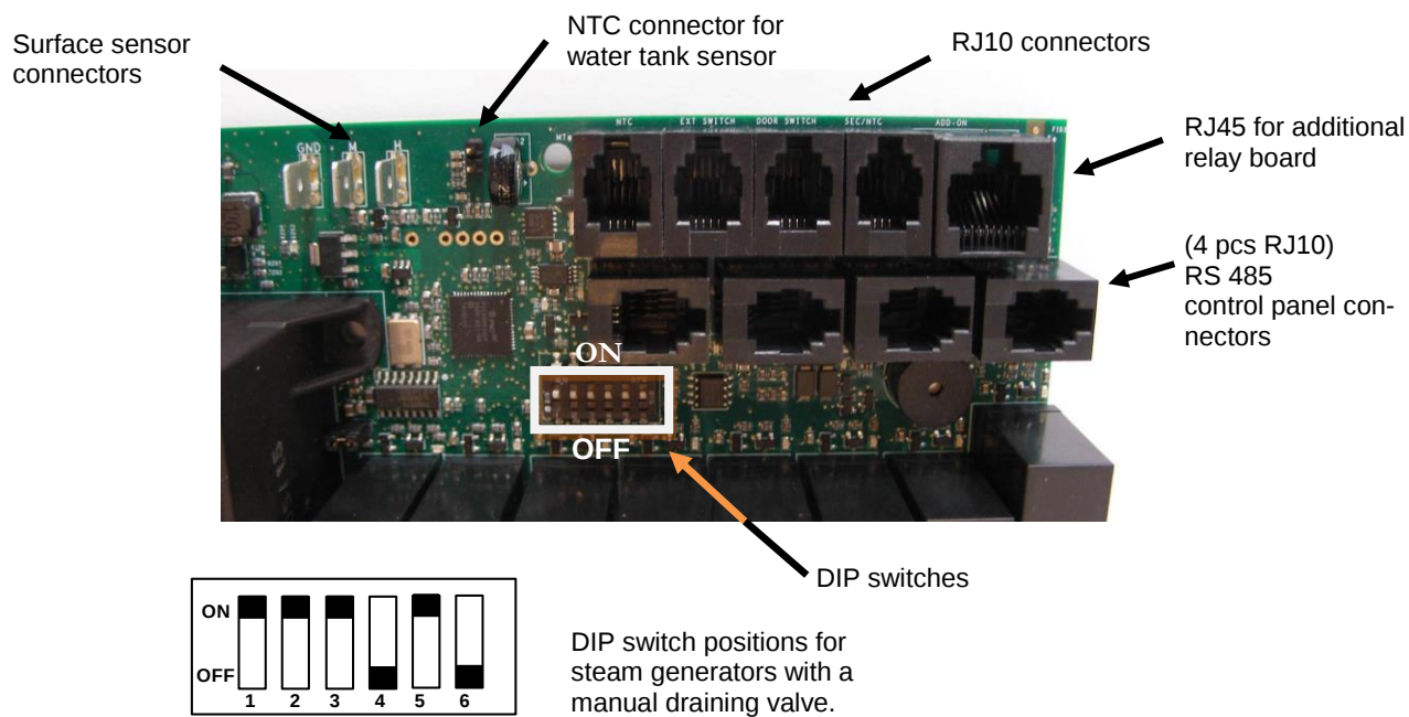
Switch diagram
