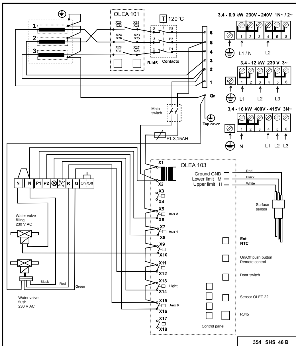
Switch diagram
